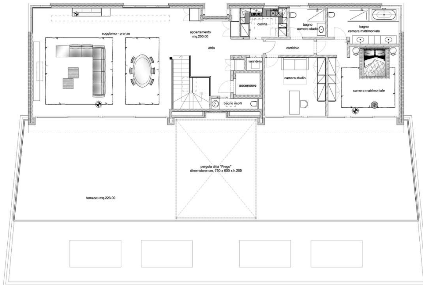
PIANTA - FLOOR PLAN
